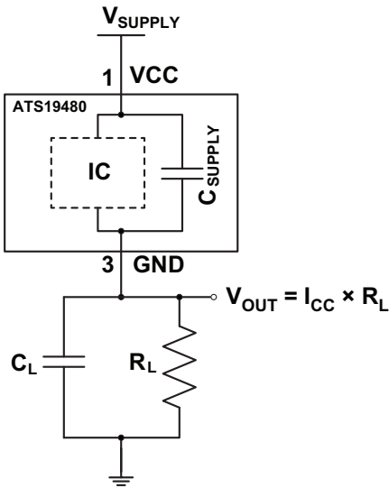
Figure 1: Typical Application Circuit
