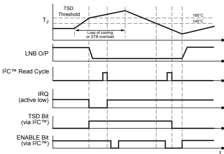
Figure 9: IRQ and Fault Clearing in Response to Thermal Shutdown (TSD). If the junction temperature rises above 165°C (typ), the LNB output will be shut off, a thermal shutdown fault (TSD) will be latched in the Status Register, and the IRQ pin will transition low. After a TSD fault, the LNB output does not respond to the Enable (ENB) bit until an I 2 C™ Read cycle is executed to report and clear the TSD fault. After a successful I 2 C™ Read, the IRQ pin transitions high and the ARG81300 can be re-enabled, provided the junction temperature is below 145°C (typ).
