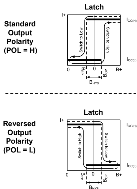
Figure 3: Hall Latch Output State vs. Magnetic Field
