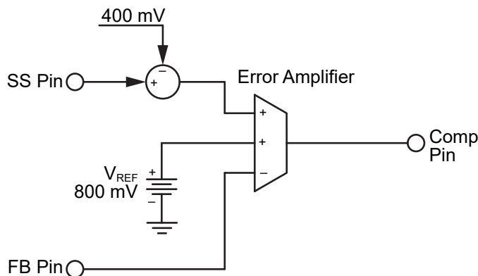
Figure 4: APM81911 Error Amplifier
