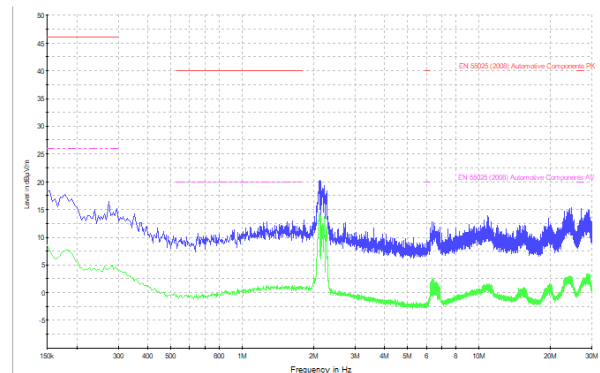
Figure 2: APM81911 Radiated Emissions from 150 kHz to 30 MHz (Monopole Antenna)
