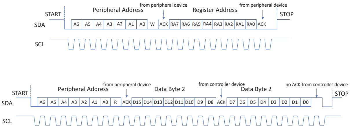
Figure 5: Read Command
