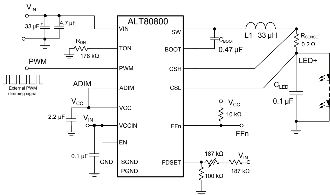
Figure 18: Application Circuit Example for ALT80800 (LED current = 1 A, 500 kHz)
