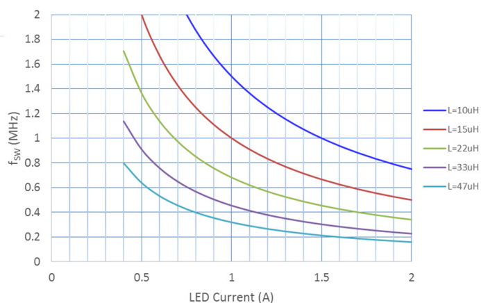
Figure 16: Minimum switching frequency vs. LED current, given different inductance used ( V_{IN} = 12 V, V_{OUT} = 6 V, ripple current = 20%)
