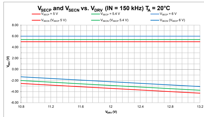
(b) IN = 150 kHz / 50% Duty Cycle, C_{OUT} = 1 nF
