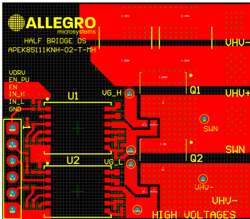
Figure 11: Example PCB Layout
