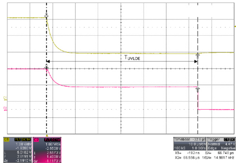
UVLO Enable Time ( t_{UVLOE} ) V_{CC} 5 V to 3 V fall time = 1.5 \mu\text{s} , C_L = 1 nF
