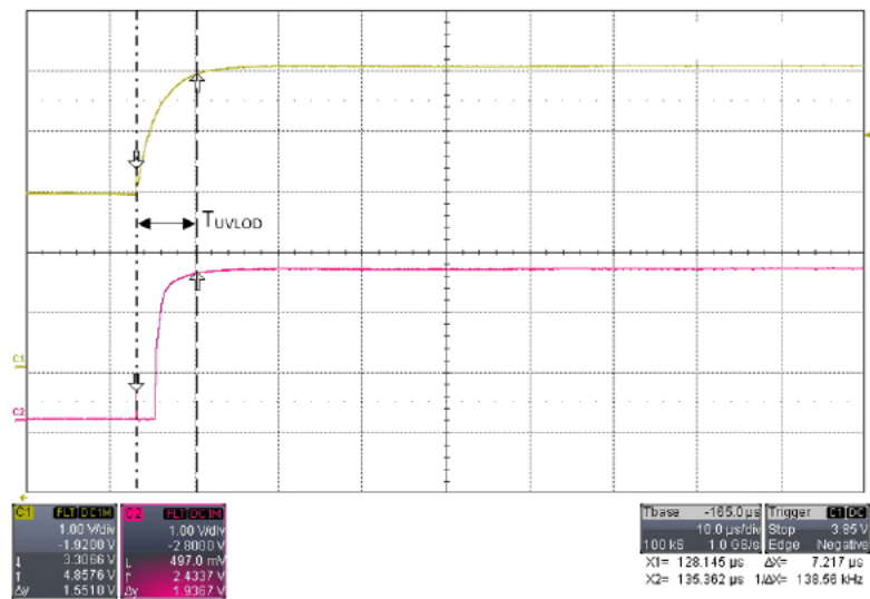
UVLO Disble Time ( t_{UVLOD} ) V_{CC} 3 V to 5 V recovery time = 1.5 \mu\text{s} , C_L = 1 nF
