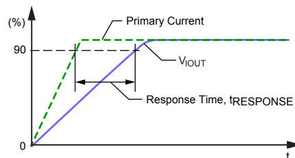
Figure 5: Response Time
