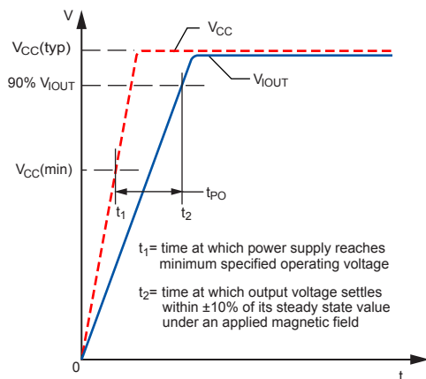
Figure 3: Power-On Time
