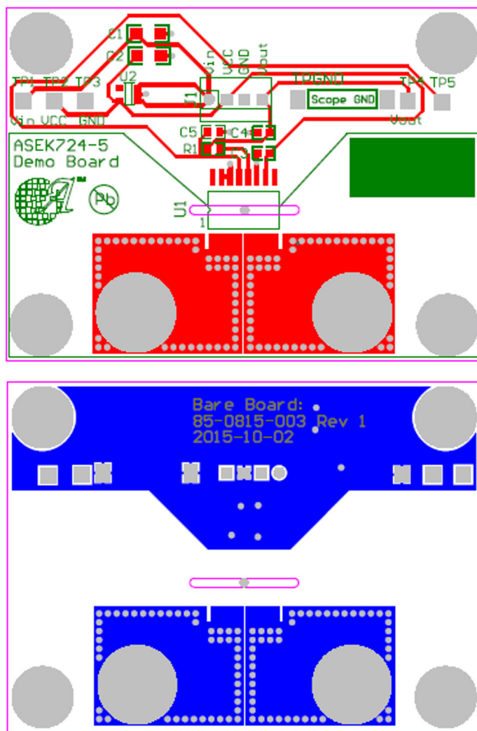
Figure 8: Top and bottom layers for ASEK724/5 MA evaluation board
