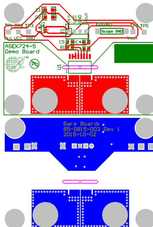
Figure 5: Top and Bottom Layers for ASEK724 Evaluation Board
