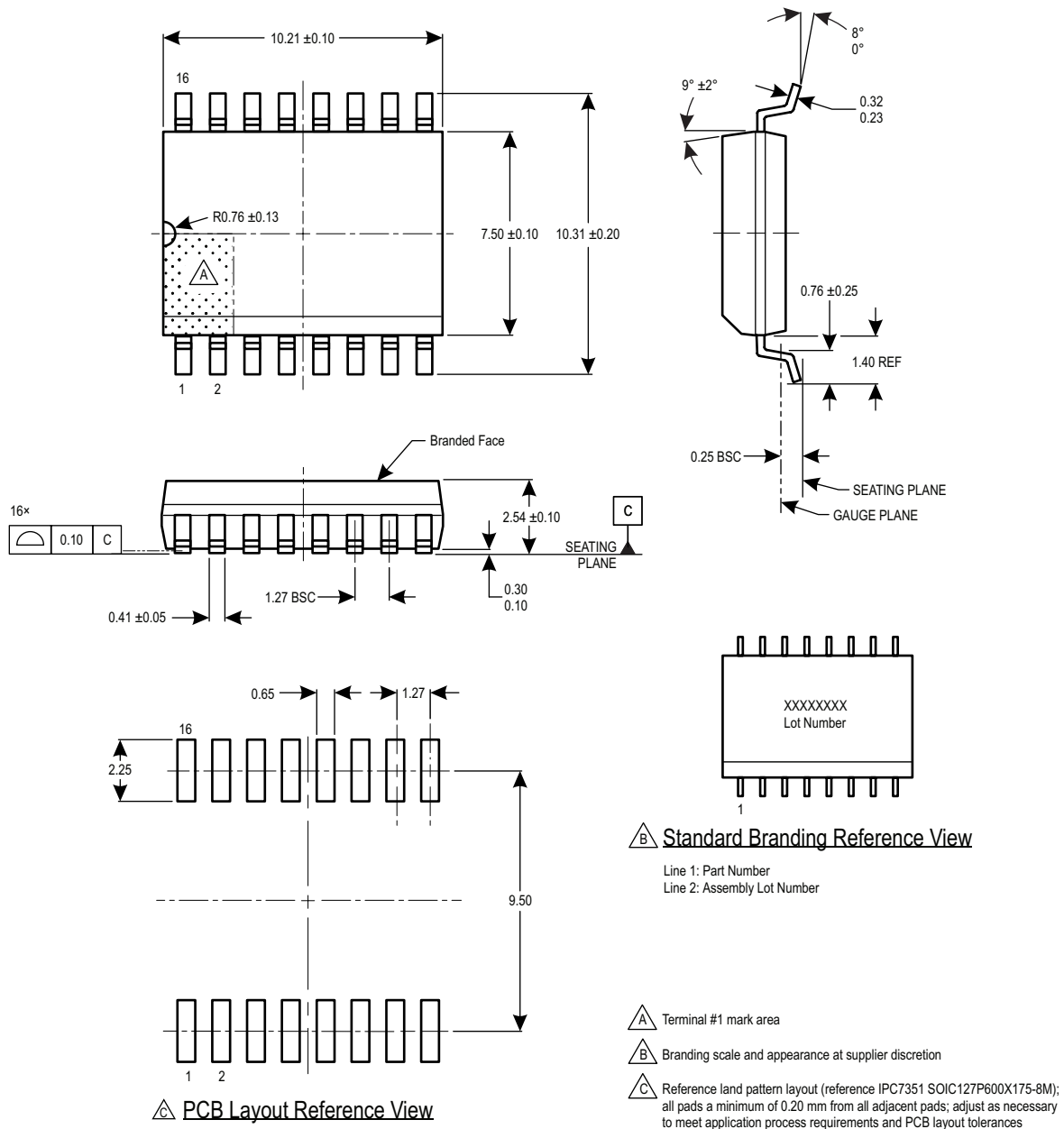
Figure 11: Package MA, 16-pin SOICW
