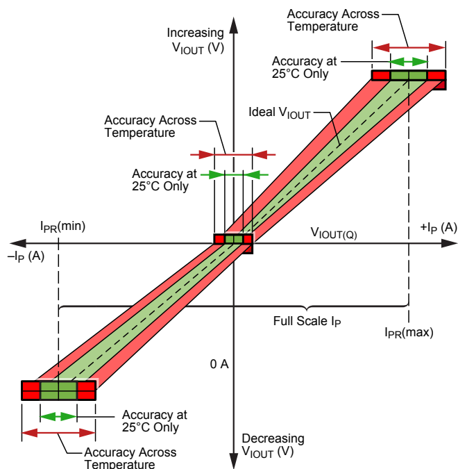
Figure 8: Output Voltage versus Sensed Current
