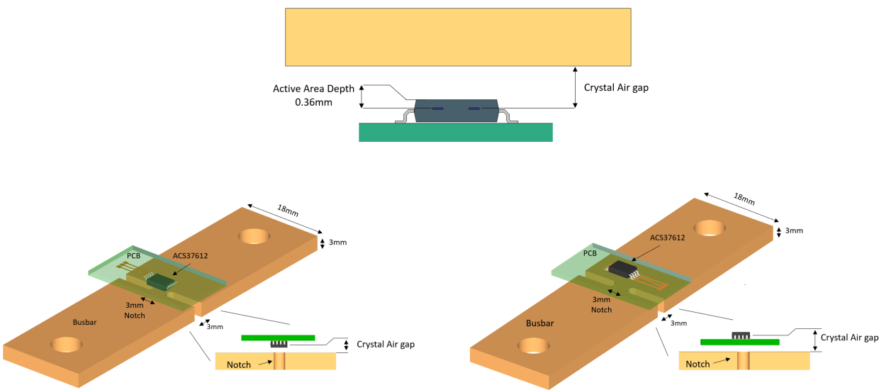
Figure 19: Busbar current sensing application – reference busbar design
