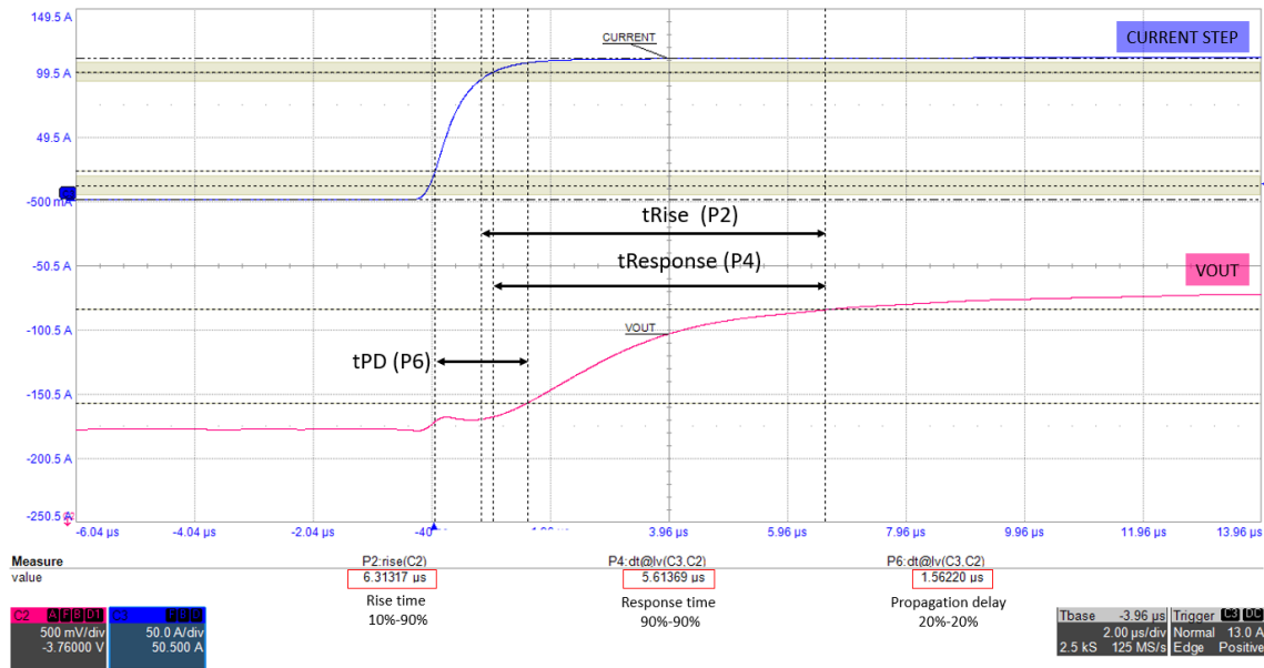
Figure 9: Response time, rise time, and propagation delay on 3.5 mm Reference PCB.
