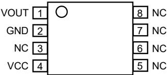
Figure 5: Pinout Diagram
