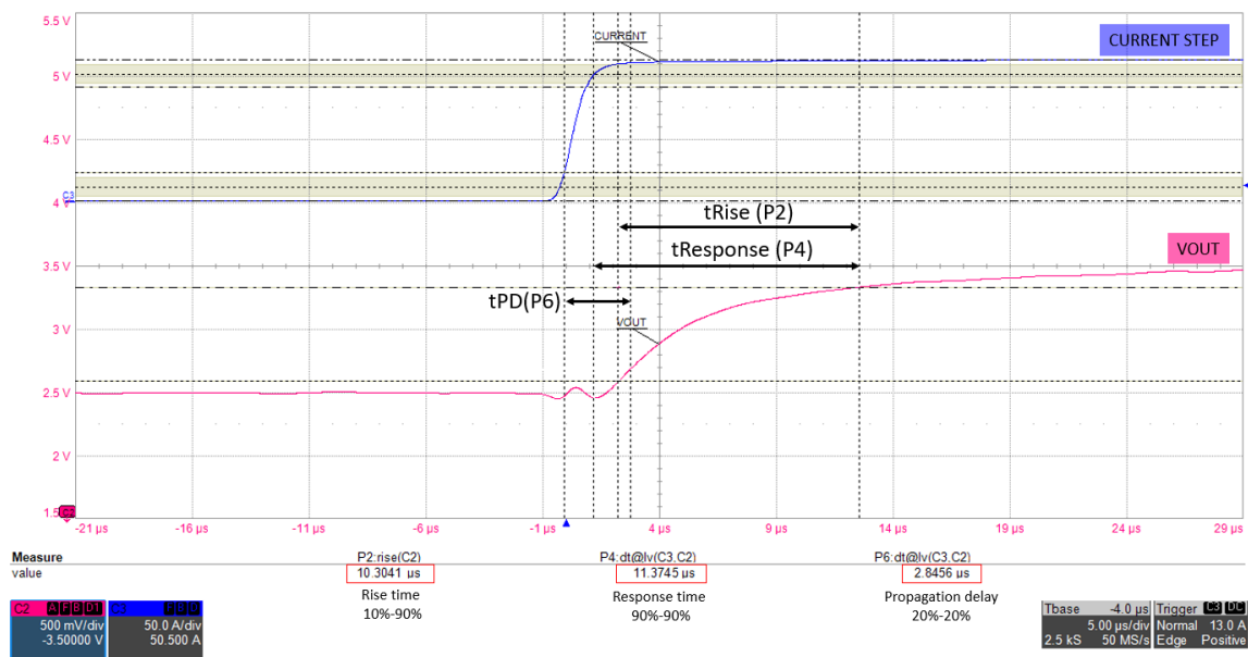
Figure 10: Response time, rise time, and propagation delay on Reference Busbar.
