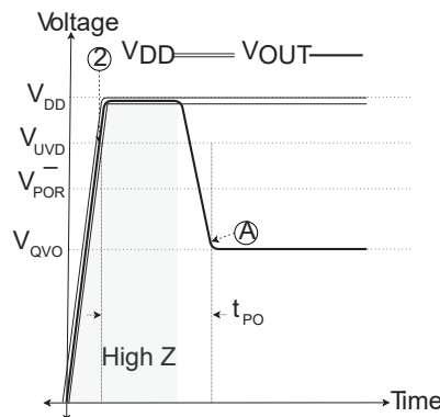
Figure 7: t_{PO} behavior UVD enabled, R_{L\_VOUT} = \text{Pull-Up}
