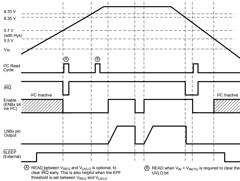
Figure 14a. I 2 C and \overline{\text{IRQ}} operate down to V IN > V REG (V REG is 5.25 V typical), LNBx and BOOSTx operate from V IN(th) . When V IN exceeds V REG (5.25 V typical), \overline{\text{IRQ}} transitions low because of the UVLO fault, and an I 2 C Read sequence will clear the \overline{\text{IRQ}} fault. While powering down, when V IN falls below V UVLO , \overline{\text{IRQ}} becomes low, LNBx and BOOSTx turn off, and I 2 C becomes inactive when V IN falls below V REG .
