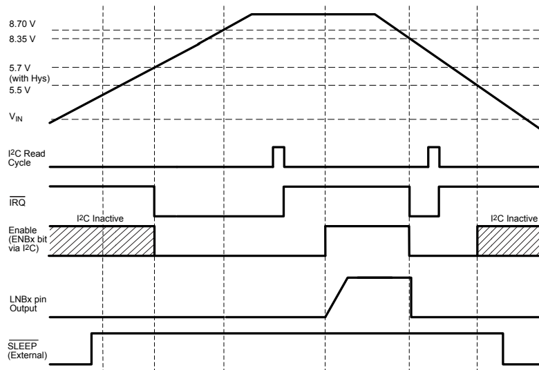
Figure 14b. \overline{\text{IRQ}} is cleared when V IN is already above V IN(th) . As the ENBx bit is already set high, LNBx starts rising immediately after an I 2 C Read sequence.
