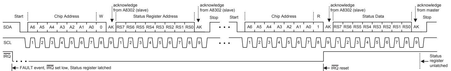
Figure 12. I2C™ Interface Read from Status register sequence. The \overline{\text{IRQ}} pin is reset to high when the A8302 acknowledges it is being read. The Status register is unlatched when the master acknowledges the status data from the A8302.
