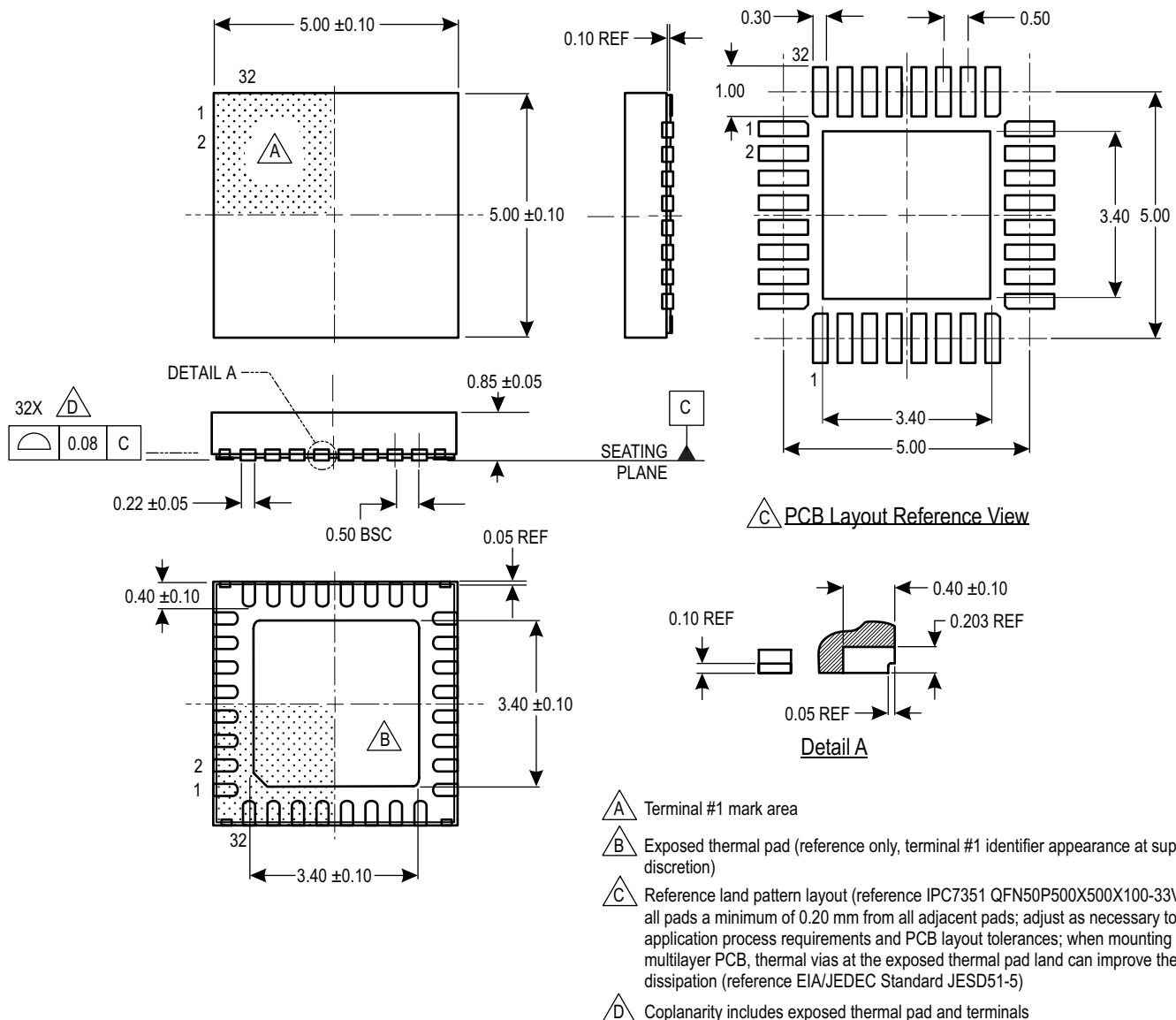
Figure 32: 32-Pin 5 mm × 5 mm QFN with exposed thermal pad and wettable flank (suffix ET)
