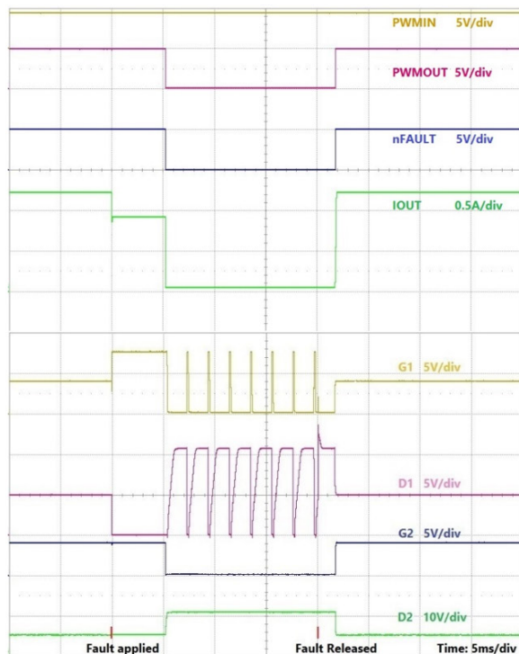
Figure 11: Open LED Fault on D1 in FULL mode. MODE = High (left), MODE = Low (right). Fault on channel 1.
