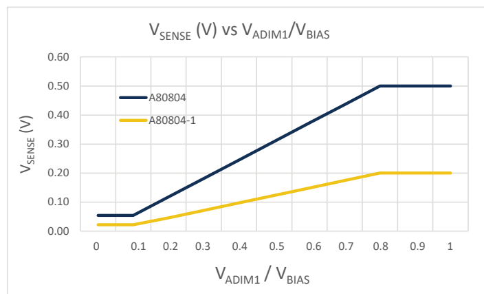
Figure 4: Effect of ADIM1 on V_{SENSE}
