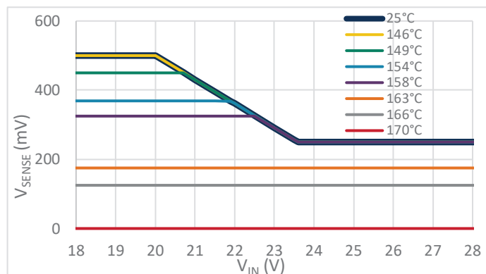
Figure 21: Combined Effect of V_{IN} Derating and Thermal Derating
