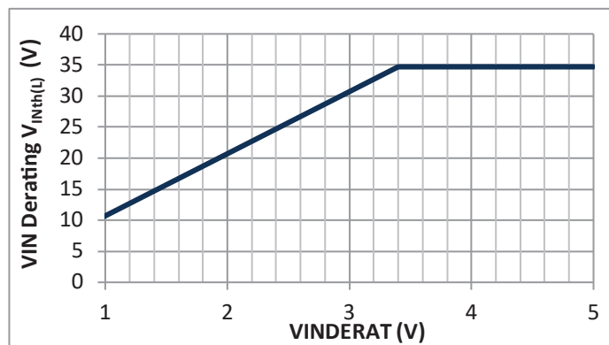
Figure 18: V_{VINDERAT} Voltage versus V_{IN} Derating Threshold
