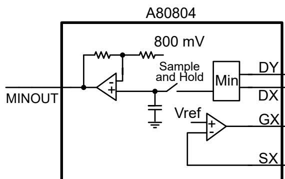
Figure 8: Block Diagram of MINOUT Block
