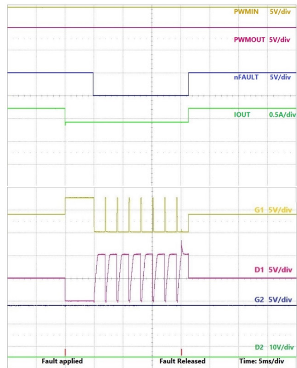
Figure 11: Open LED Fault on D1 in FULL mode. MODE = High (left), MODE = Low (right). Fault on channel 1.
