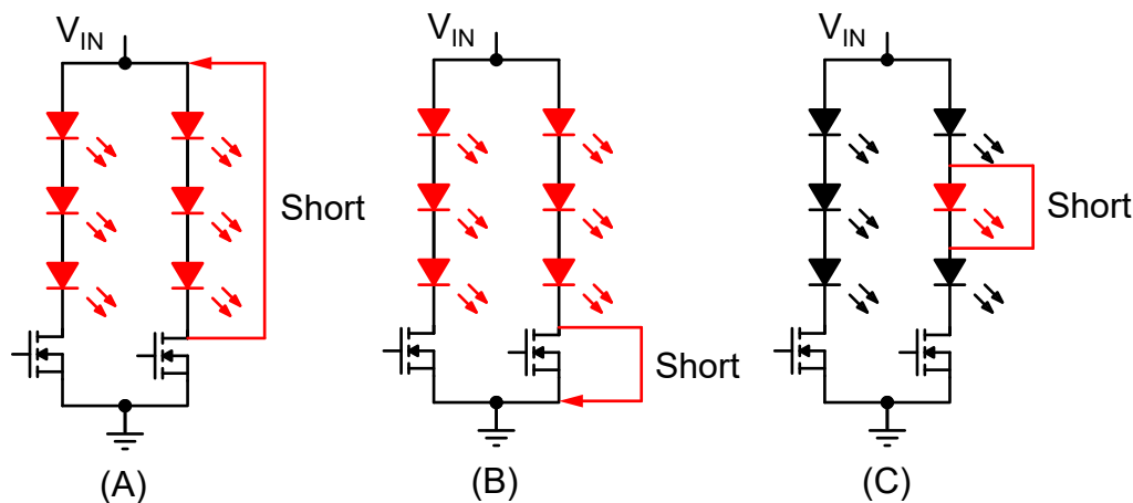
Figure 14: Short-Circuit Protection
