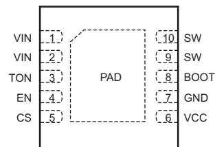
Package EJ Pinouts
