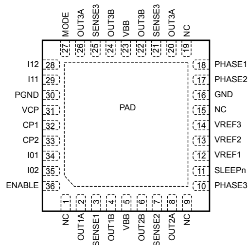
Pinout Diagram
