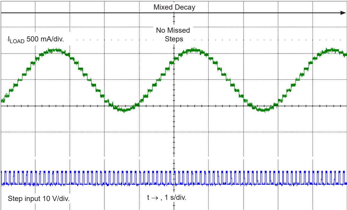
Figure 4: Continuous Stepping Using APFD (ROSC Pin Grounded)
