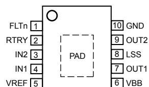
LY Package (A4952)
