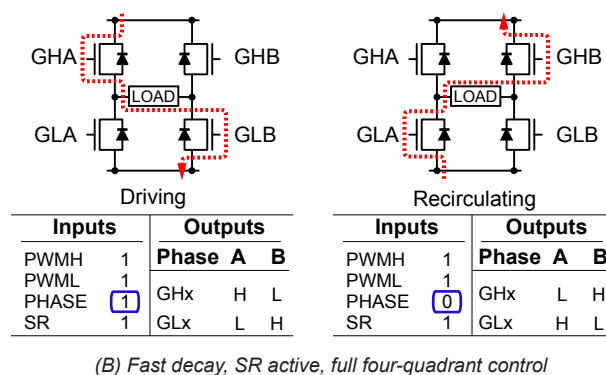
Figure 2: Fast Decay Power Bridge Current Paths
