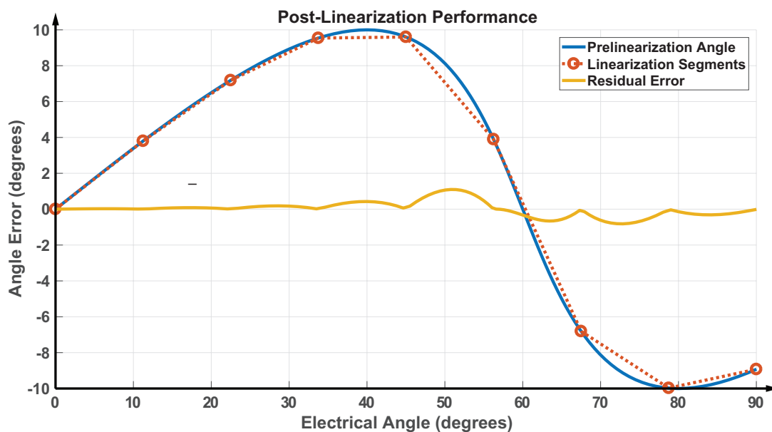
Figure 8: Post-Linearization Error
