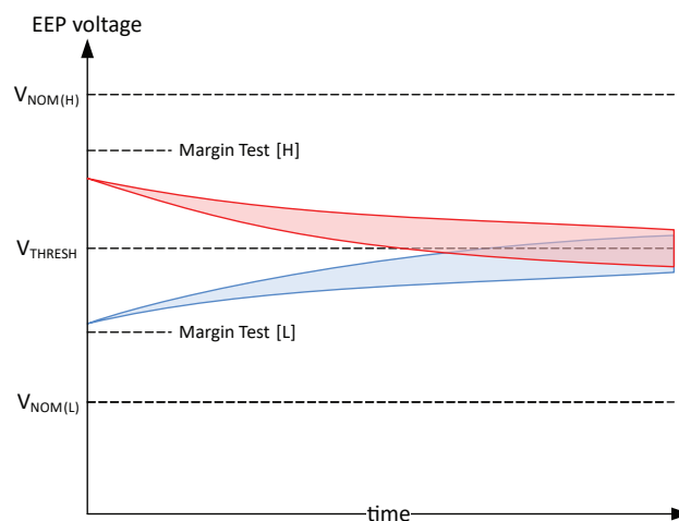
Figure 32: Example of failing programming voltages
