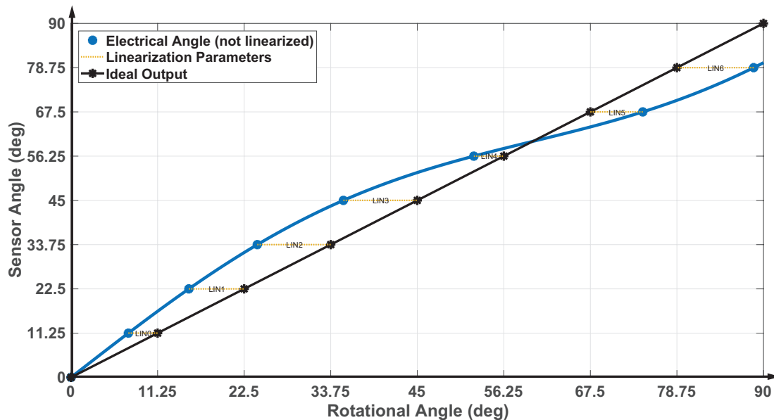
Figure 7: Linearization Example
