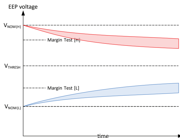
Figure 31: Example of passing programming voltages
