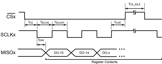
Figure 16: A33002 SPI Interface Timings Output
