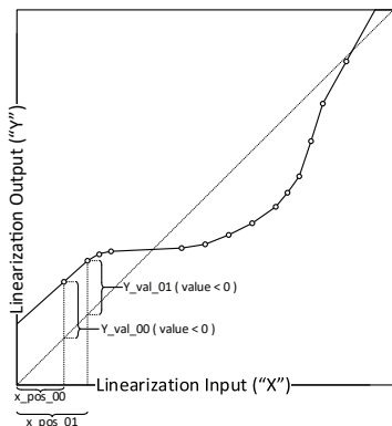
Figure 14: Variable-Segment Linearization
