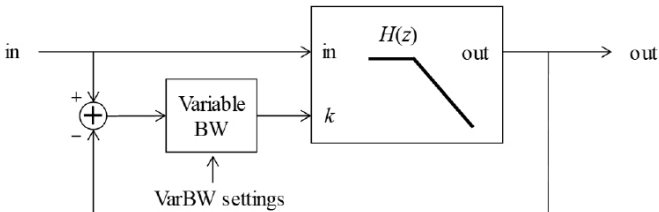
Figure 5: Low-Pass Filter
