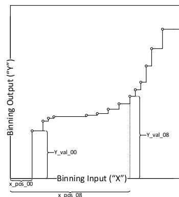
Figure 15: Variable-Segment Binning
