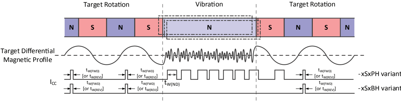
Figure 15: Vibration Behavior
