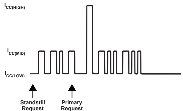
Figure 15: I_{CC(HIGH)} Pulse-Truncating Standstill Pulse Example
