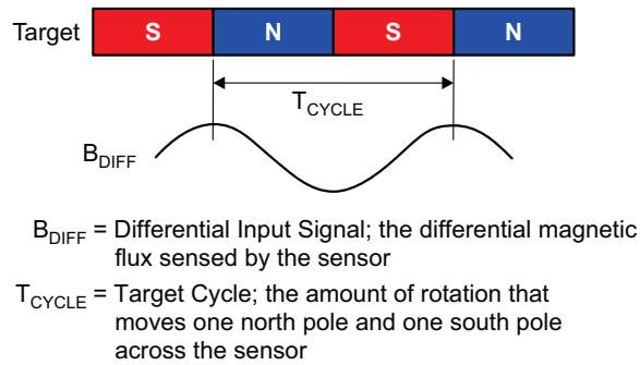
Figure 5: Definition of T_{CYCLE}
