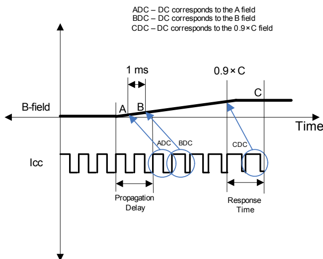
Figure 2. Definitions of Propagation Delay and Response Time
