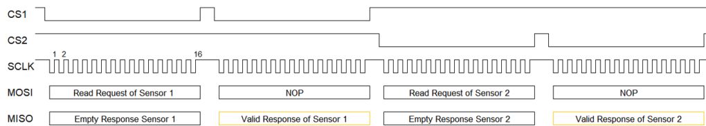
Figure 75: Implementation of SPI Using 16- or 17-Bit Packets; Valid Data, IER Flag Still Asserts
