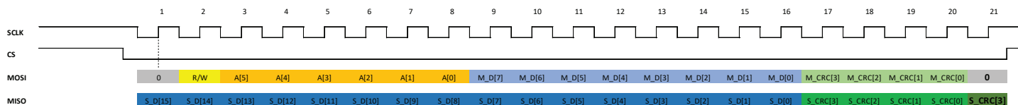
Figure 73: 21-Bit SPI Packet Format
