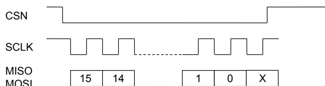
Figure 46: 16-Bit SPI Transaction
