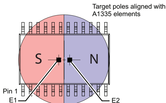
Figure 12: Orientation of Magnet Relative to Primary Die and Secondary Die
