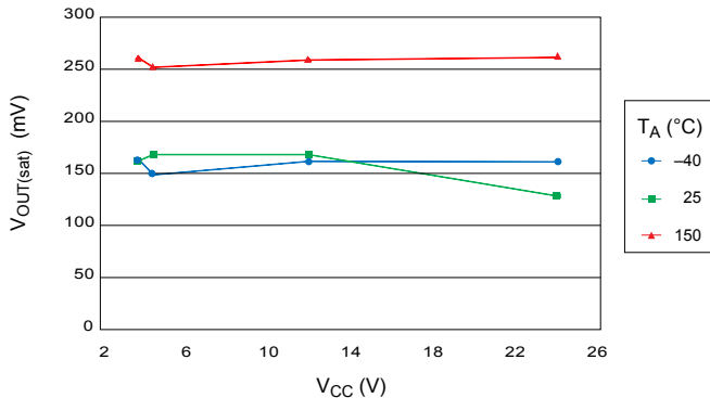
Average Output Saturation Voltage versus Supply Voltage
