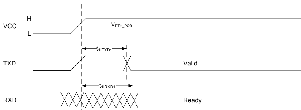
Figure 10.6-1. UART wake-up timing after V_{RTH\_POR}
