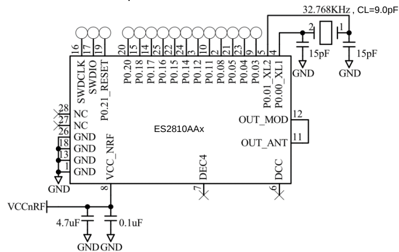
Internal LDO setup with external 32.768kHz X'tal
