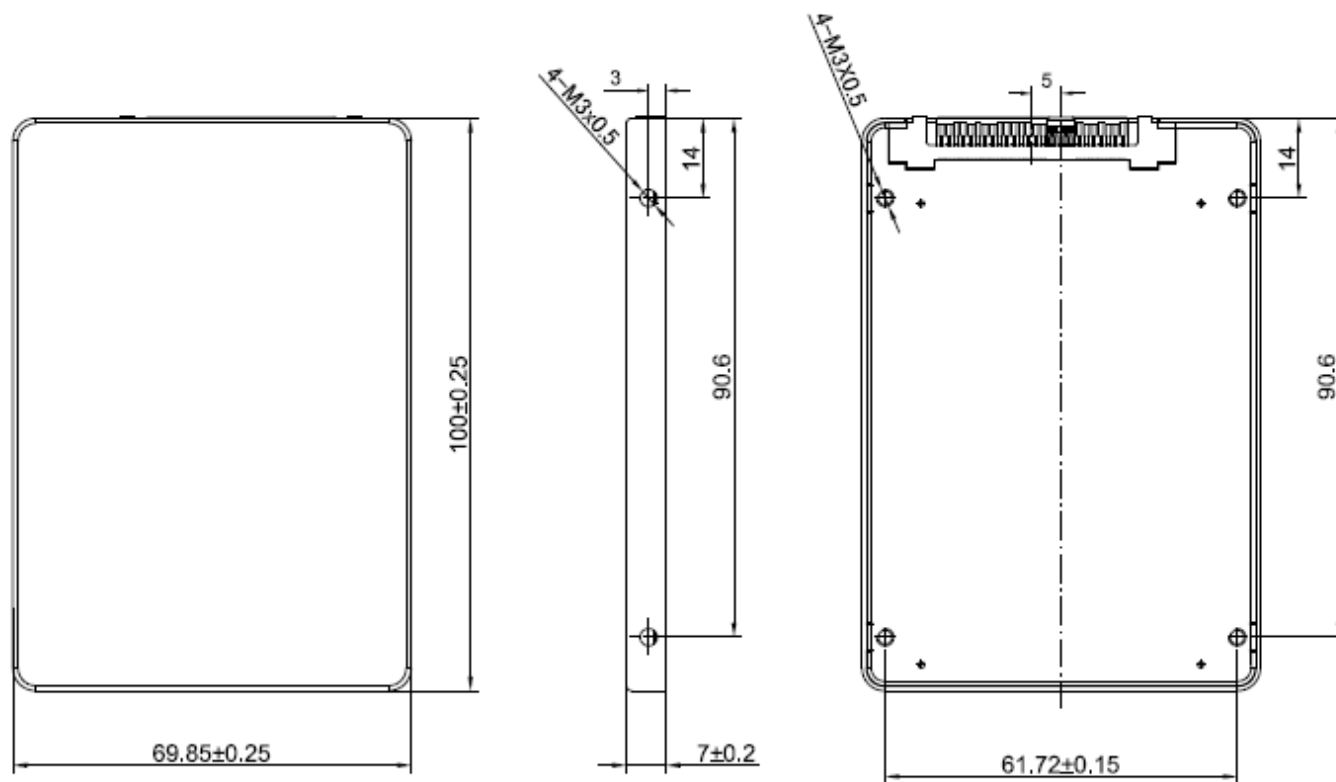
Figure 2: U.2 physical dimension diagram
