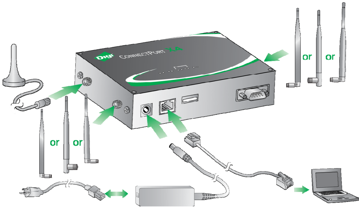
Figure 2: Connecting Hardware
