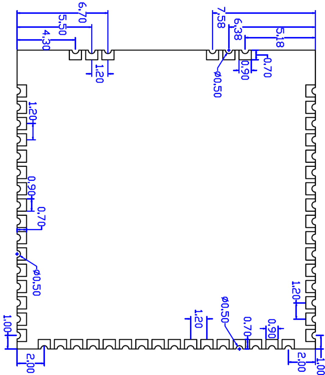
Bottom View
