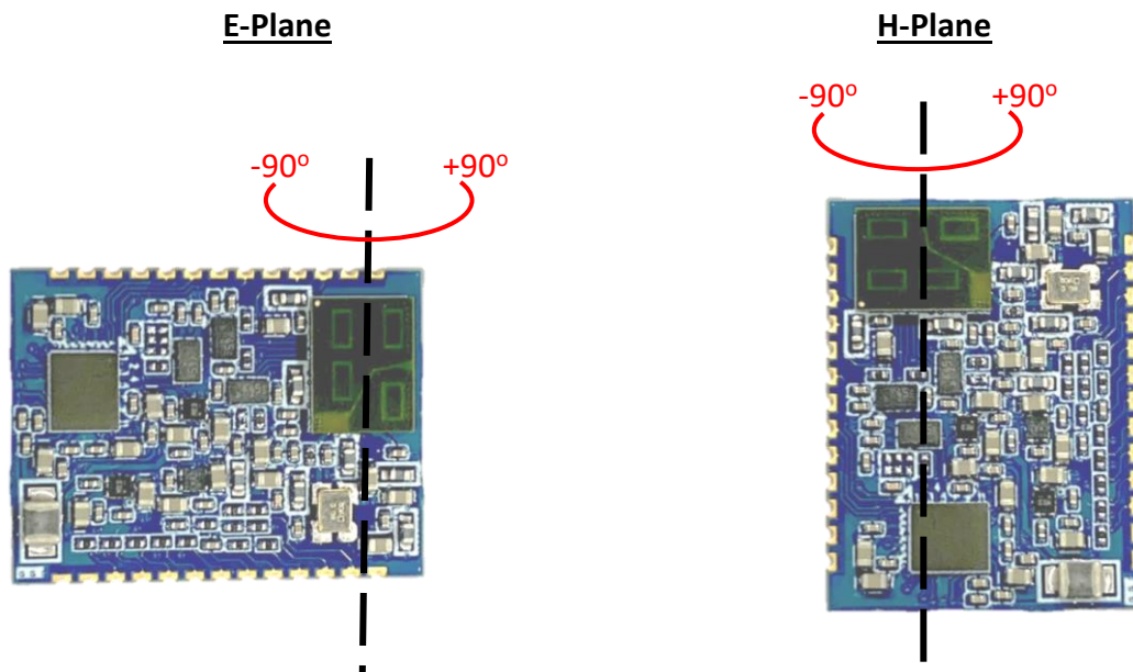
Figure 3-1. Antenna Setup
