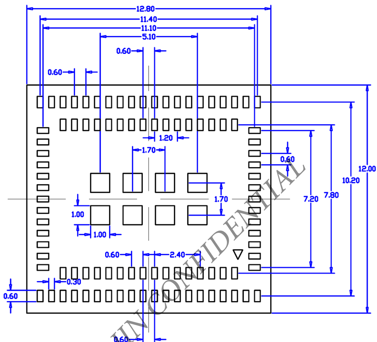
Figure 9-2. Module pad dimensions
