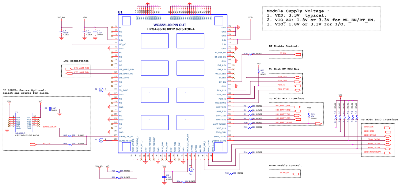
Figure 5-1. WG3221-00 module reference circuit
