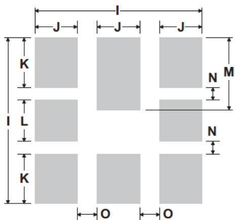
PCB Footprint Top View
