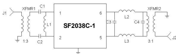
Test Circuit
