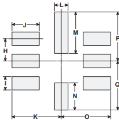
PCB Footprint
