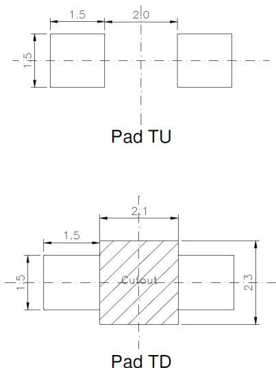
Recommended Soldering Pattern
