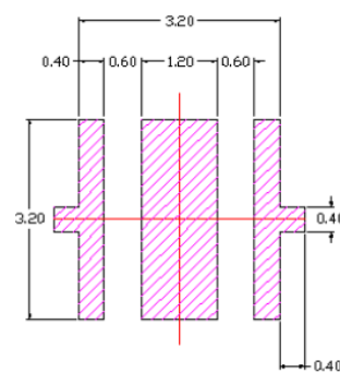
Recommended Stencil Pattern
