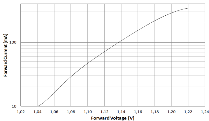
U_F - I_F characteristic
