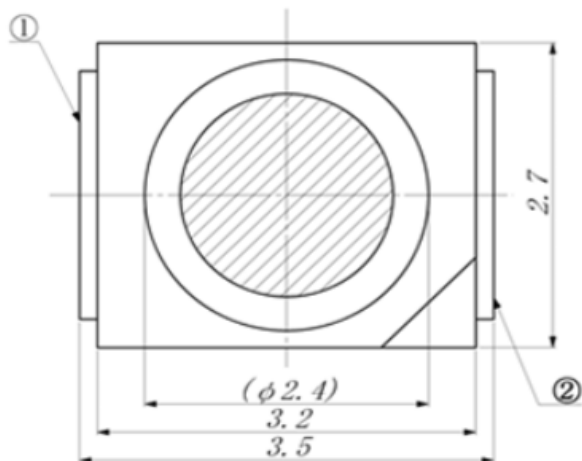
① Cathode
