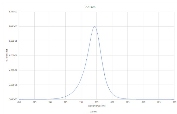
Spectral Response
