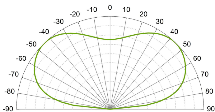
Radiation pattern
