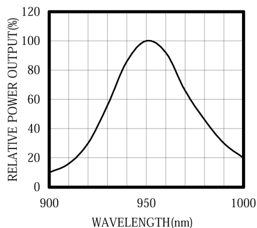
SPECTRAL OUTPUT
