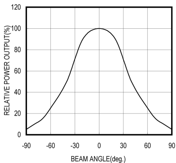
RADIATION PATTERN
